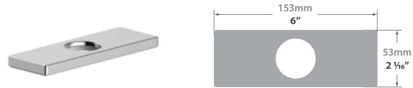
■ 6" cover plate for lavatory faucet
