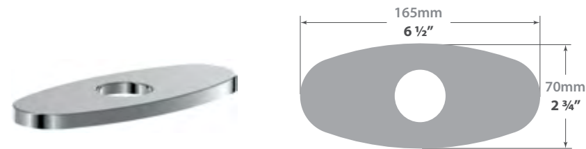
■ 6" cover plate for lavatory faucet
